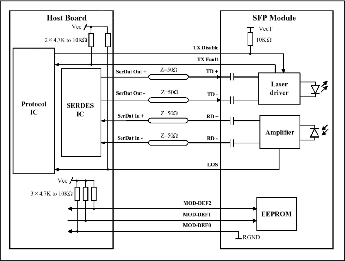
Block Diagram of Transceiver
